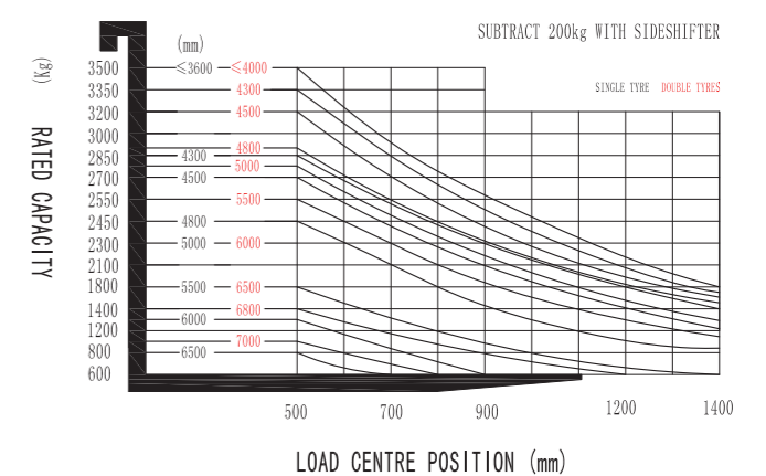
RATED CAPACITIES AND LOAD CENTERES GRAPH
